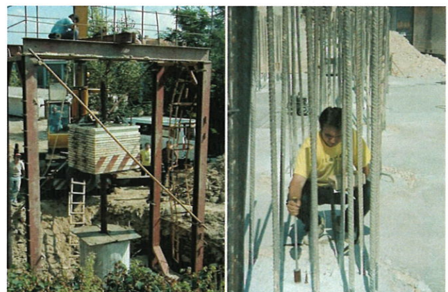
Fig. 1. Dynamic testing of the pile capacity and integrity of pile columns
